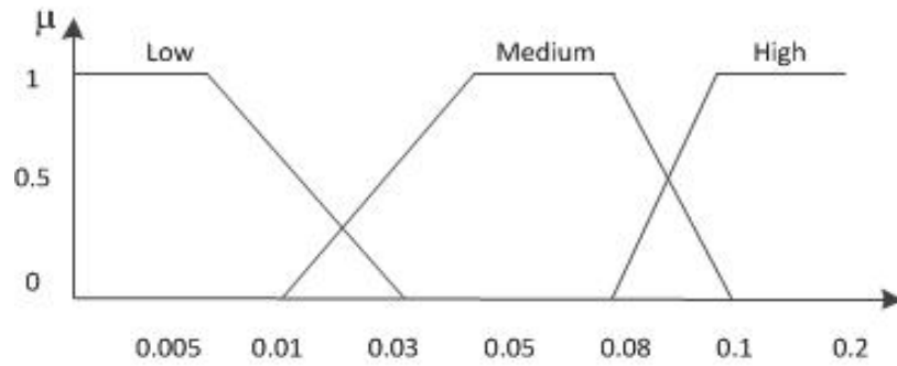
Fig. 4: Membership function of packet loss rate
