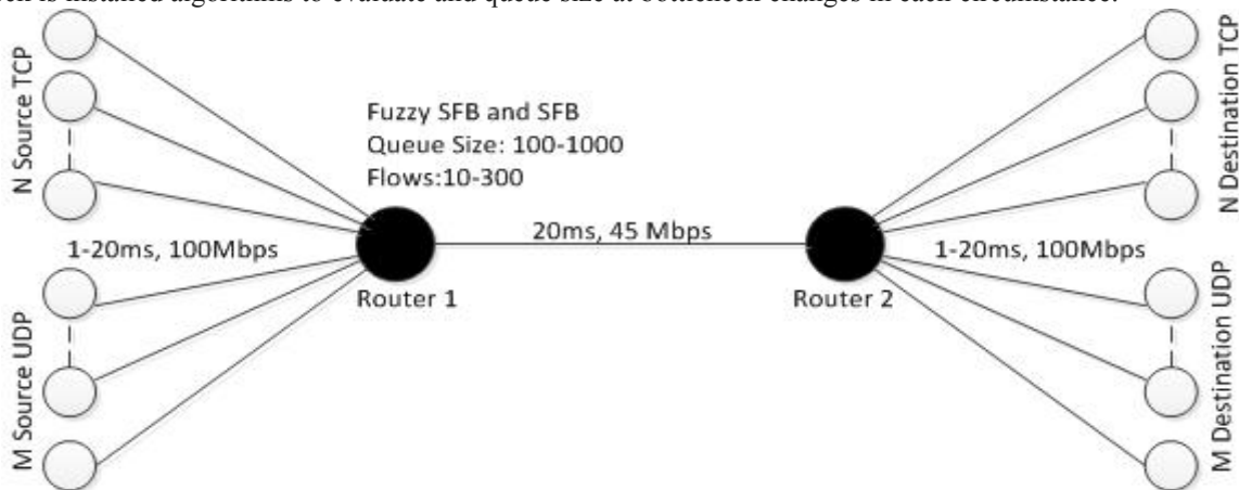
Fig. 7: Network simulation model
