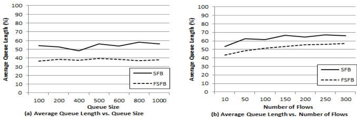
Fig. 11: The usage of the active queue management mechanisms
