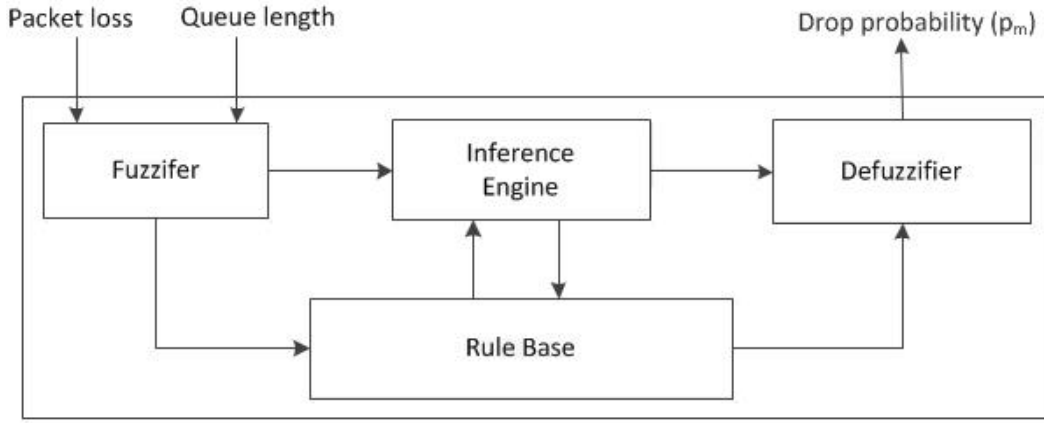
Fig 3: Architecture of fuzzy inference system
