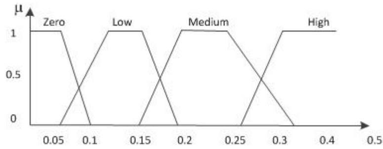
Fig. 6: Membership function of packet loss probability
