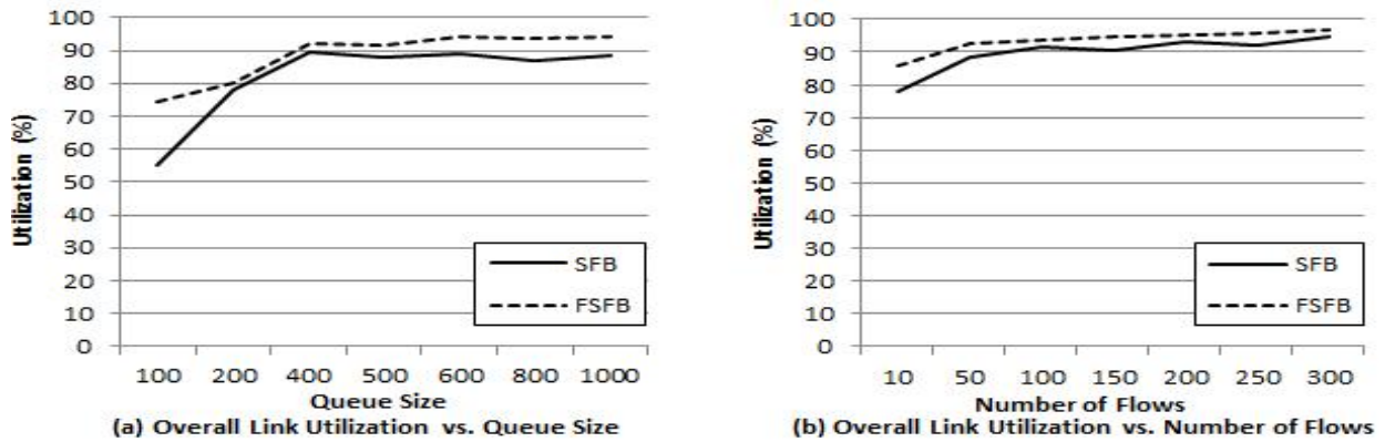
Fig. 9: The usage level of the transmission line of mechanisms of active queue management
